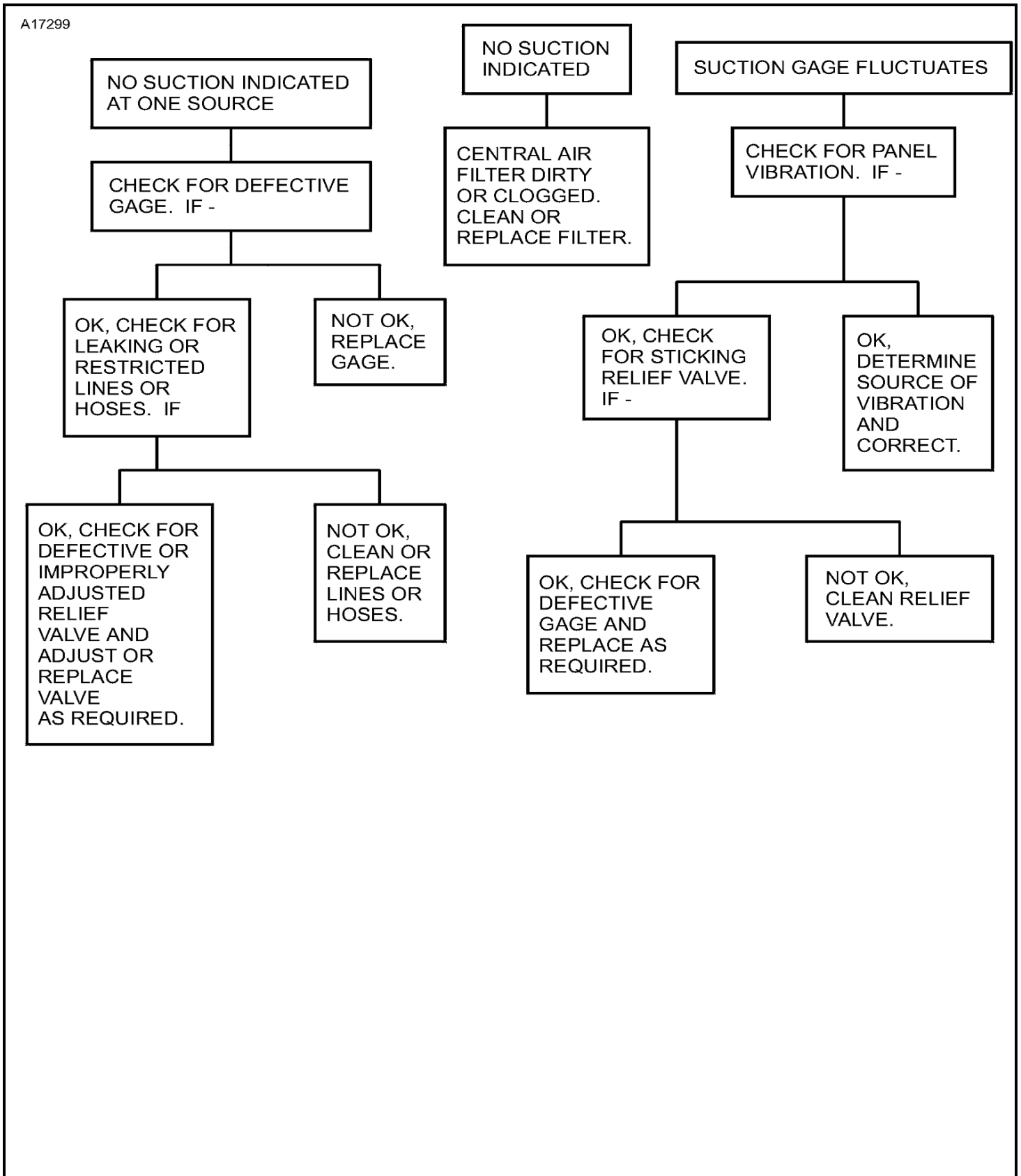
Figure 101 : Sheet 2 : Vacuum System Troubleshooting
